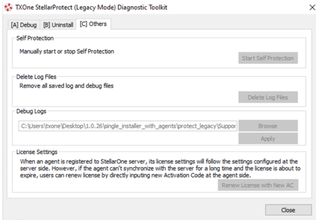
Figure 8. The TXOne Stellar Agent - Protect Edition (Windows-Legacy) Diagnostic Toolkit Debug Tab C [Others]
