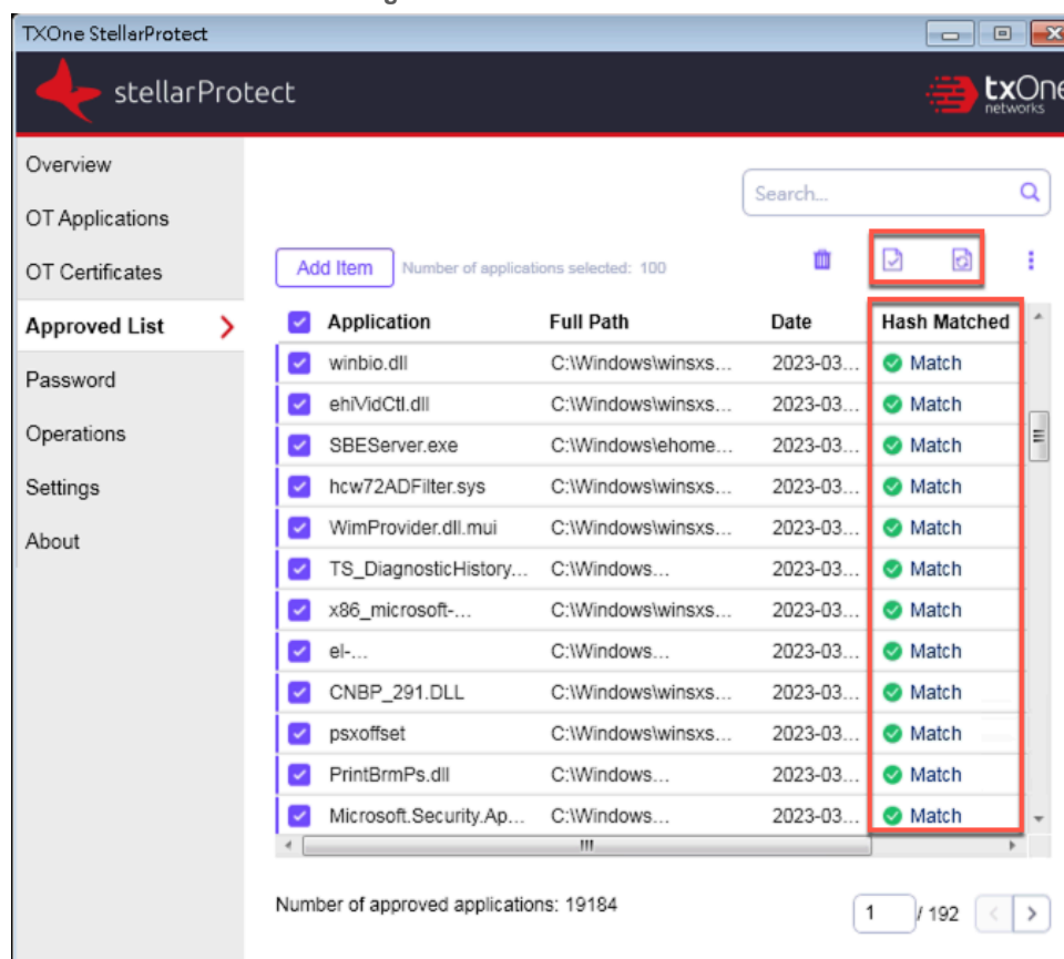
Figure 1. Hash Values Matched
