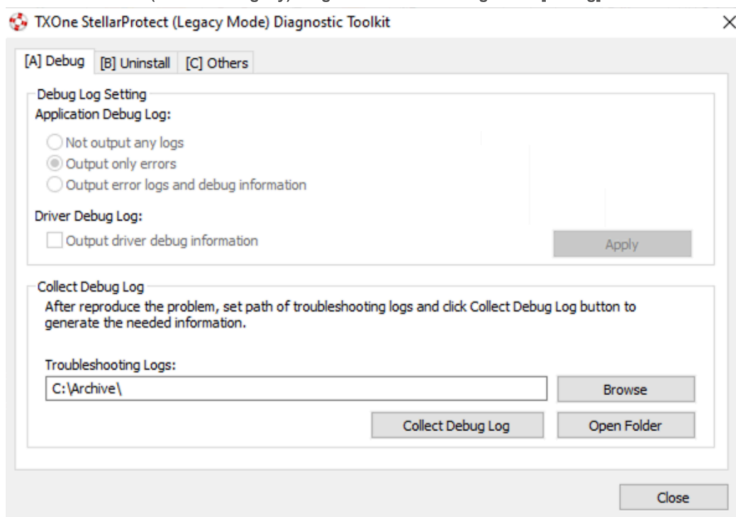
Figure 6. The TXOne Stellar Agent - Protect Edition (Windows-Legacy) Diagnostic Toolkit Debug Tab A [Debug]
